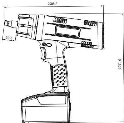
BET-80PD
